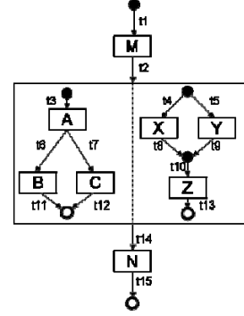
Figure 4. TPT State Machines.
